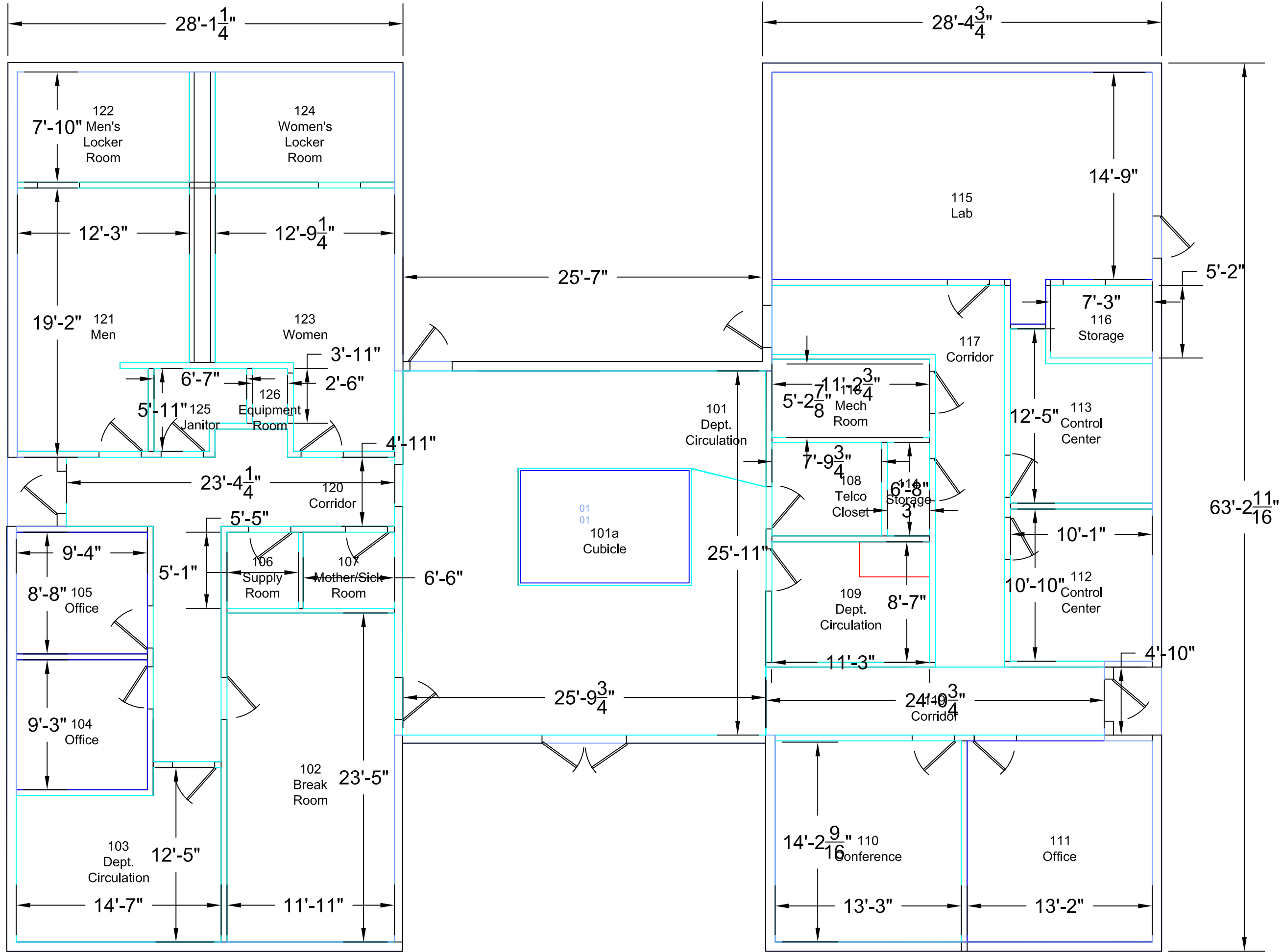
SAWS - MEDIO CREEK BUILDING # 1 REVISED: 10-03-2013
